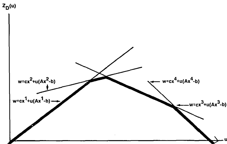
FIGURE 1. The Form of Z_D(u) .
